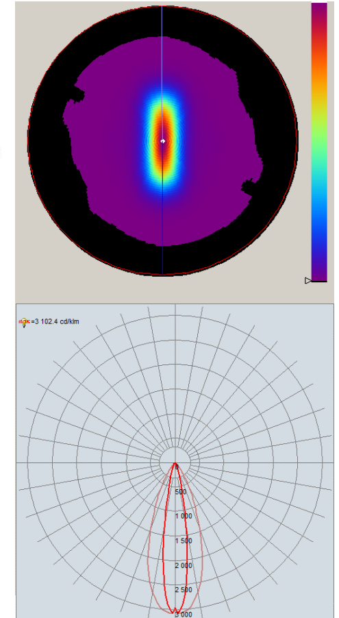
Intensity pattern
