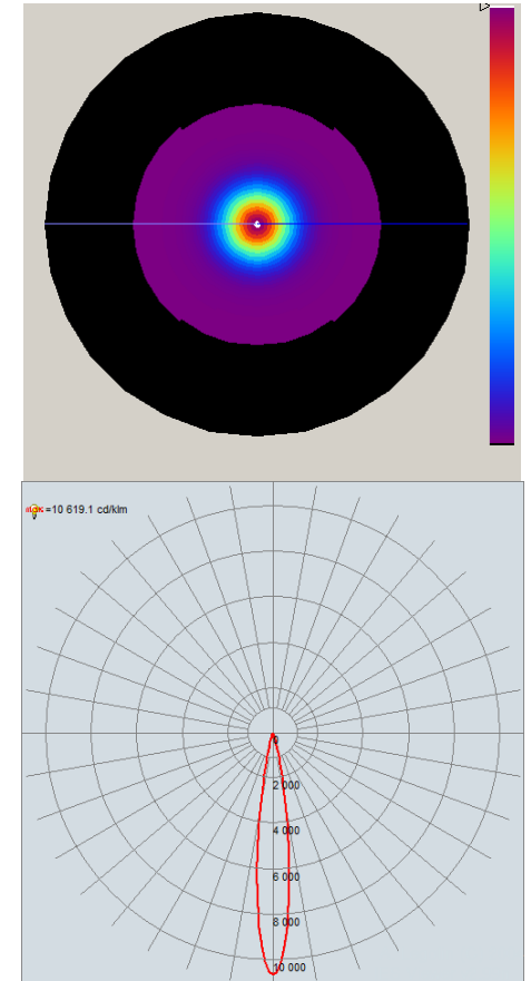
Intensity pattern
