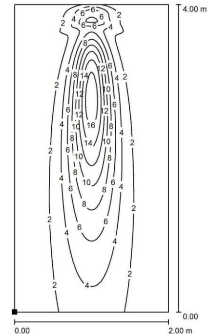
Dialux simulation
