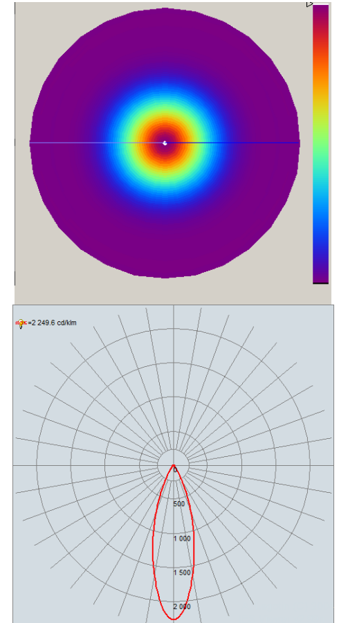
Intensity pattern
