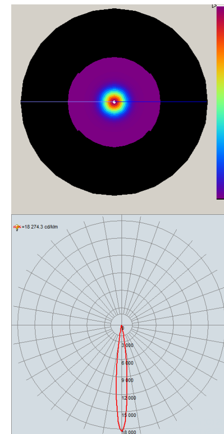
Intensity pattern
